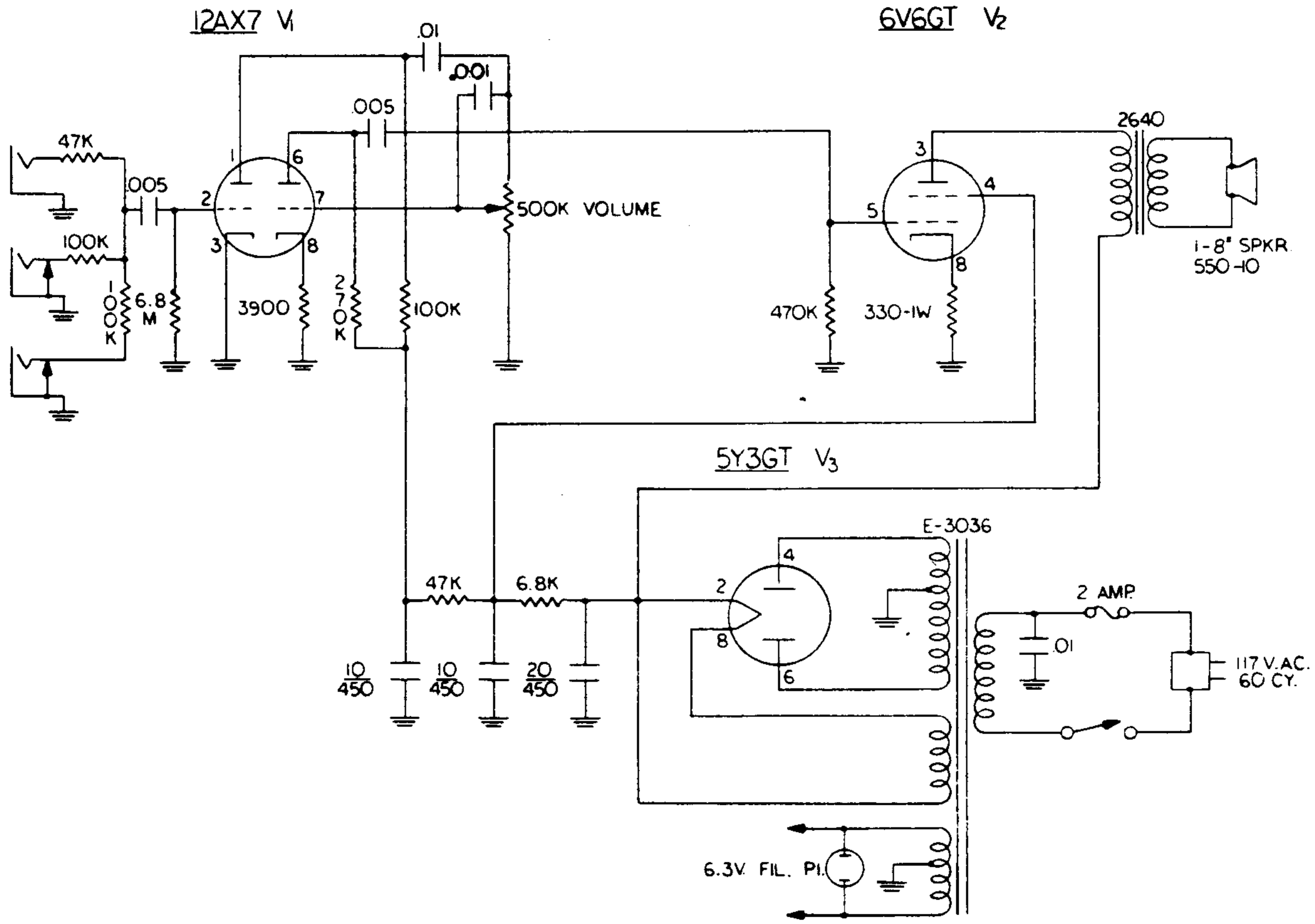
Valco Model 6150
