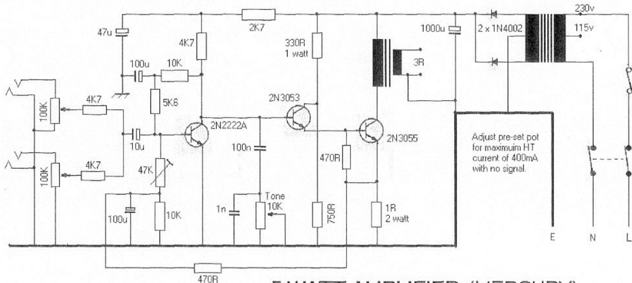
5 WATT AMPLIFIER. (MERCURY)
