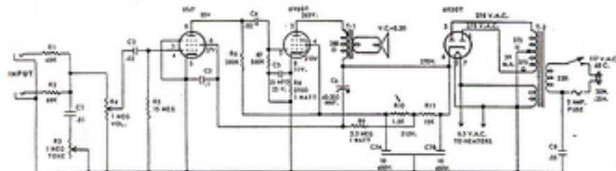
FIG. 5. SCHEMATIC DIAGRAM OF SILVERTONE CHASSIS 1331
