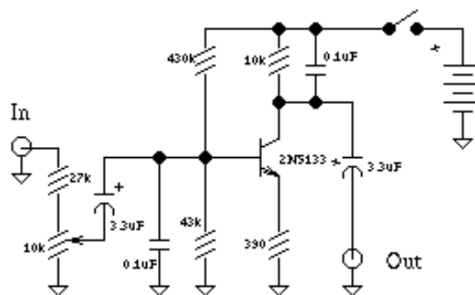
Mole/Hog's Foot (Old Version)
