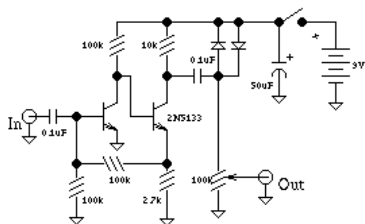
Muff Fuzz / Little Muff Pi (early)
