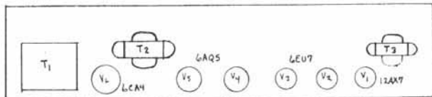
VOLTAGES TO CHASSIS WITH VTVM (117mg)
