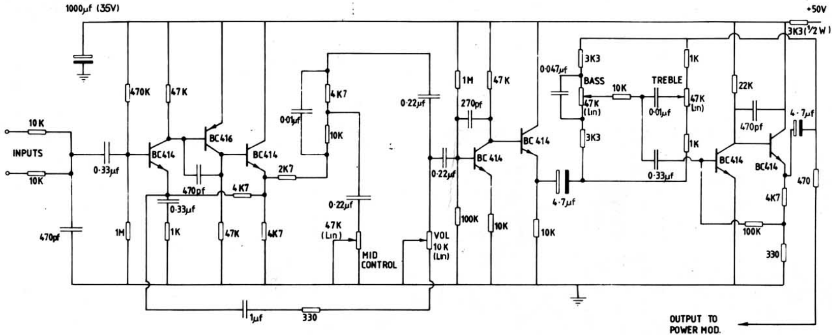
Vox Venue Bass 100 Pre-amp
