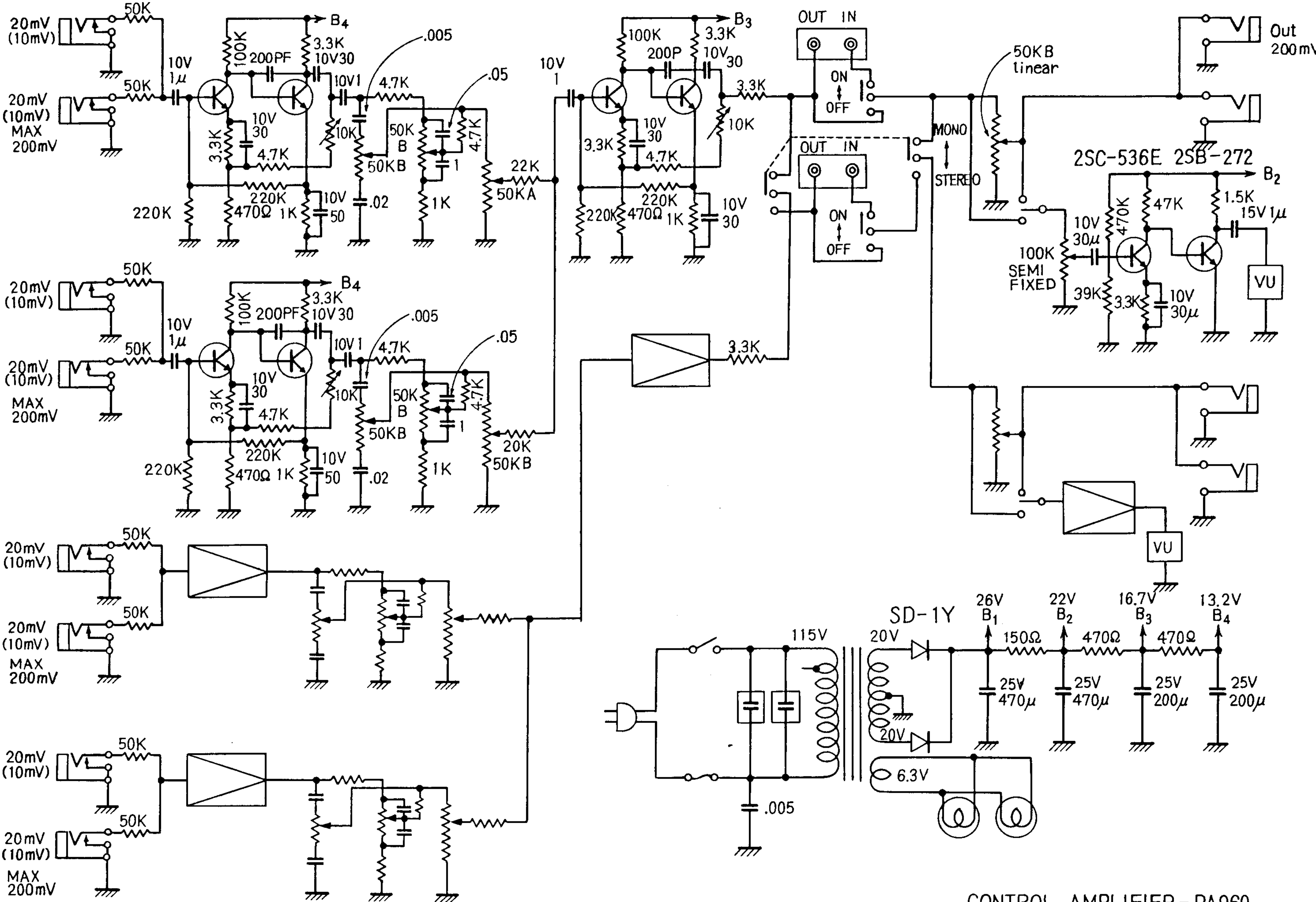
CONTROL AMPLIFIER - PA960
